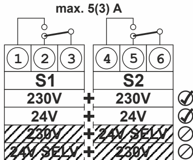
Fig. 4. Auxiliary switches
