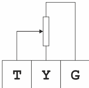
Fig. 5. Auxiliary potentiometer
