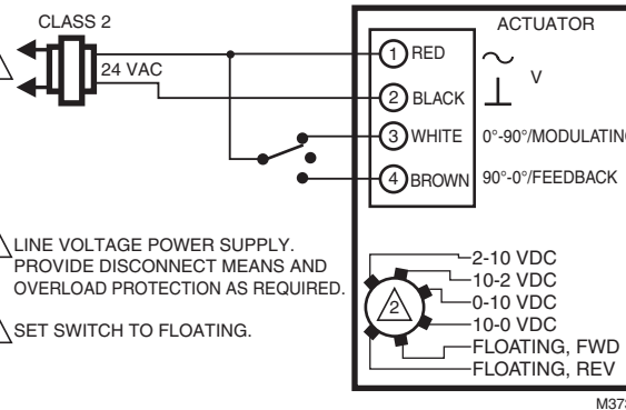
Fig. 27. MS7505 with Floating Control.
