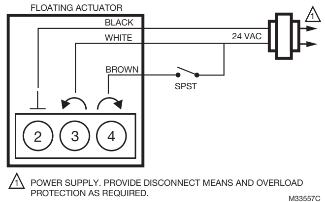
Fig. 23. MVN643 with Two Position SPST Control.
