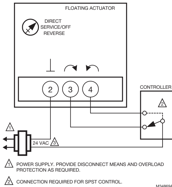
Fig. 17. MN6105 with On/Off SPDT Control.
