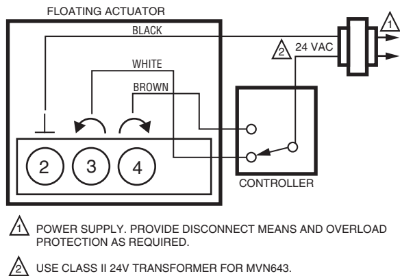
Fig. 22. MVN613 or MVN643 with Two Position SPDT Control.
