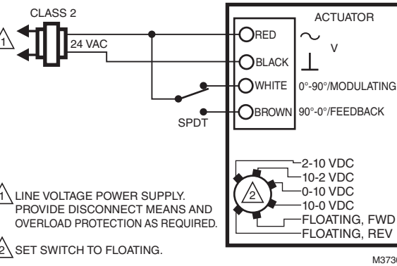
Fig. 26. MS7505 with Two Position SPDT Control.
