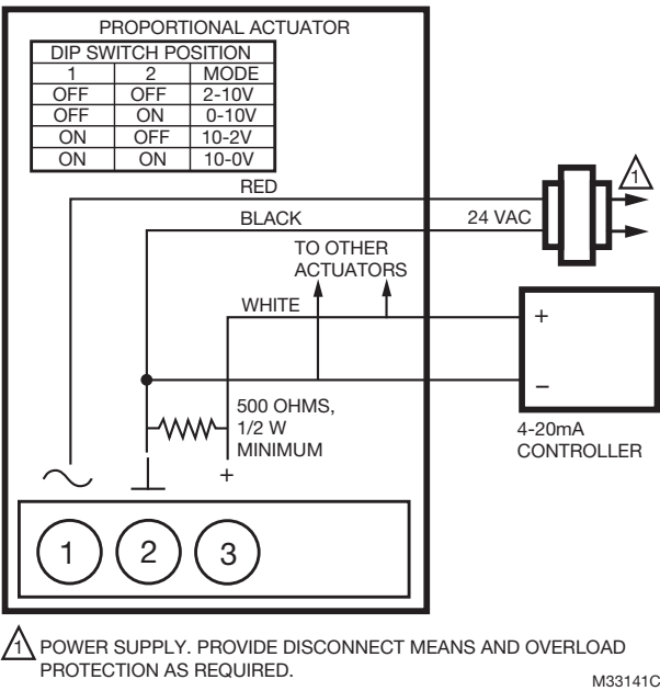
Fig. 24. MVN713 with 4-20mA Control.
