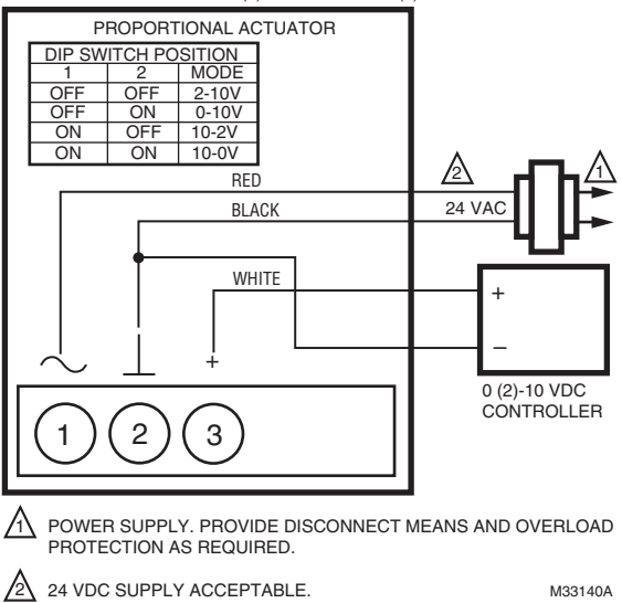
Fig. 25. MVN713 with 0(2)-10 Vdc Control.
