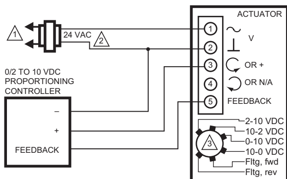
Fig. 35. MS7505 with override to full closed.
