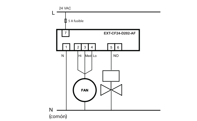
On-Off - 2 Cables
