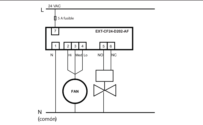
On-Off - 3 Cables
